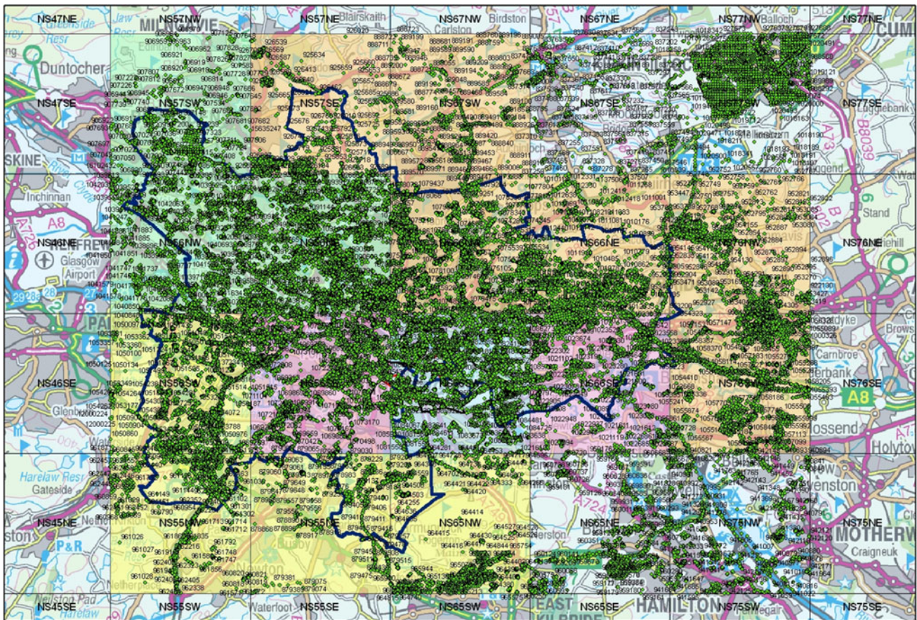
Fig. 7 Map showing the distribution of boreholes used to develop the three dimensional geological model for Glasgow, UK. Grid lines are orientated north–south and east west and are 5 km apart
