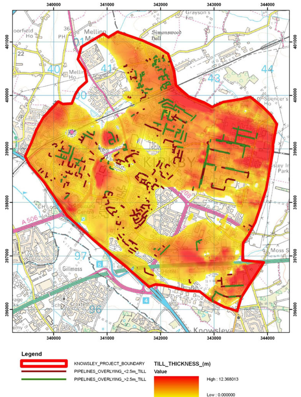
Fig. 12 Sewer locations relative to till thickness beneath them in Knowsley, Liverpool, UK. The grid lines are orientated north–south and east west and are 1 km apart. Utilities locations published with permission of United Utilities. OS topography © Crown Copyright. All rights reserved. 100017897/2008 (after Price et al. 2008b)
