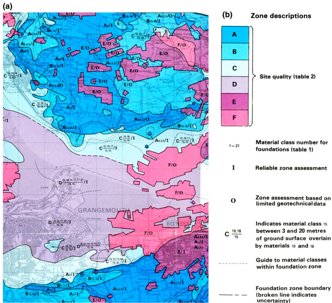
Fig. 3 a Extract from the geotechnical planning map of the upper Forth Estuary, Scotland, UK, for heavy structures. The grid lines are orientated north–south and east–west and are 1 km apart (after Gostelow and Browne 1986). b Key to the geotechnical planning map of the upper Forth Estuary, Scotland, UK, for heavy structures (after Gostelow and Browne 1986) c Ground classification scheme for
