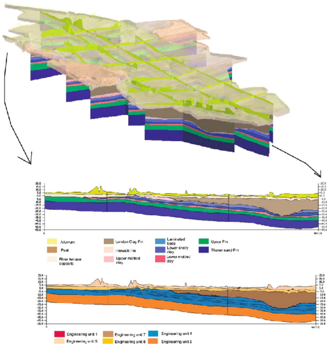
Fig. 10 3D geological model of the Lower Lea Valley, Stratford, east London, UK (site of the 2012 Olympics) with automatically generated geological and engineering geological cross-sections through the
