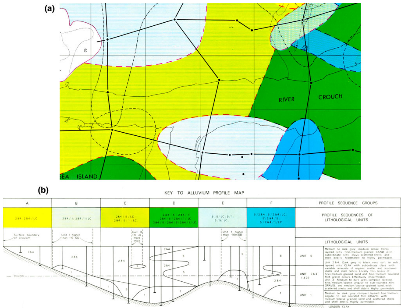
Fig. 2 a Part of a profile map of Alluvium in south-east Essex, UK. The grid lines are orientated north–south and east–west and are 1 km apart (after Anon 1977). b Key for a profile map of Alluvium in south-east Essex, UK. (after Anon 1977)
