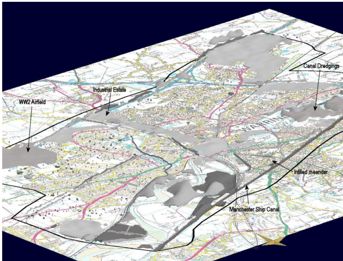
Fig. 9 3D Model of the anthropogenic deposits in Warrington, UK. (Scale as indicated by the 1 km grid on the base map; grid lines are orientated north–south, with north to the top left) [OS topography © Crown Copyright. All rights reserved. BGS 100017897/2010]
